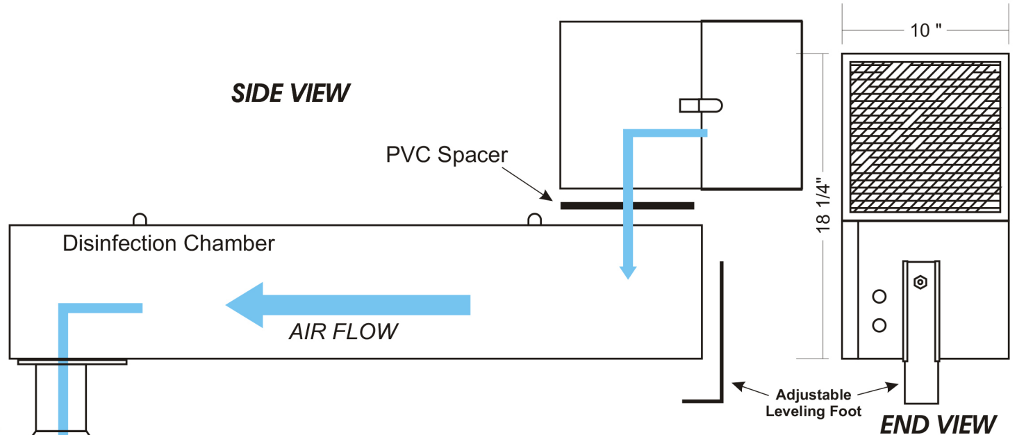
Filter/Blower Housing
